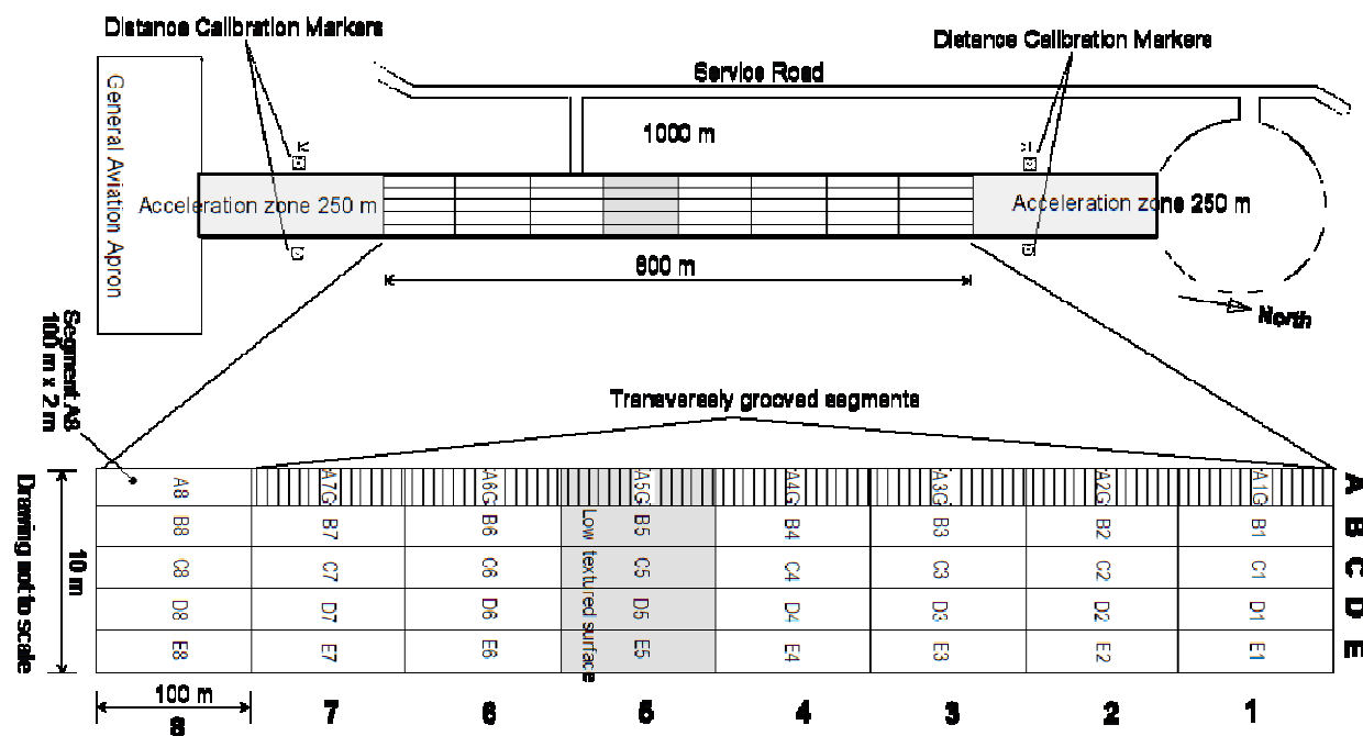
Figure 24 - Schematic drawing of the test track
