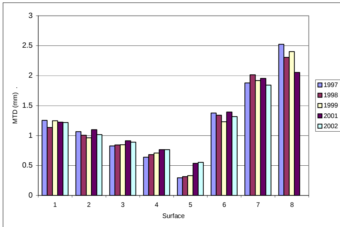
Figure 26 - Mean texture depth for OKK surfaces 1997 - 2002
