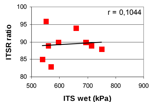
Figures 11a and 11b: ITSR ratio as a function of indirect tensile strength of dry and wet asphalt concrete samples.
