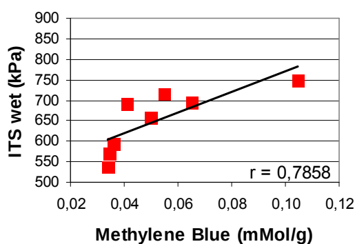
Figures 10a and 10b: Indirect tensile strength of dry and wet asphalt concrete samples as a function of methylene blue value of the filler.
