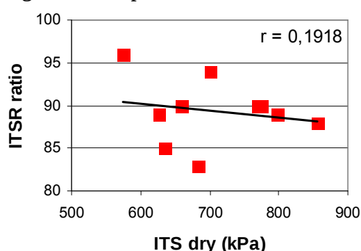
Figures 11a and 11b: ITSR ratio as a function of indirect tensile strength of dry and wet asphalt concrete samples.
