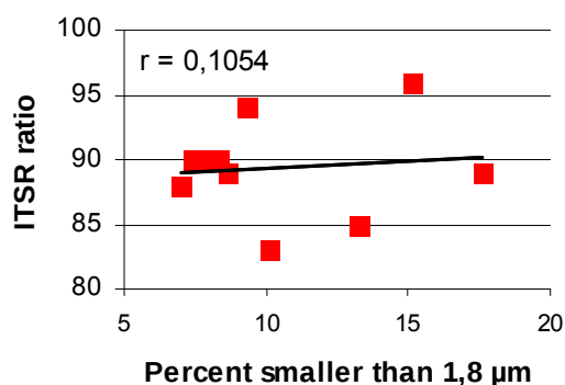
Figure 12a: ITSR ratio of asphalt concrete mixes as a function of percent of filler smaller than 1,8 \mu\text{m} .
