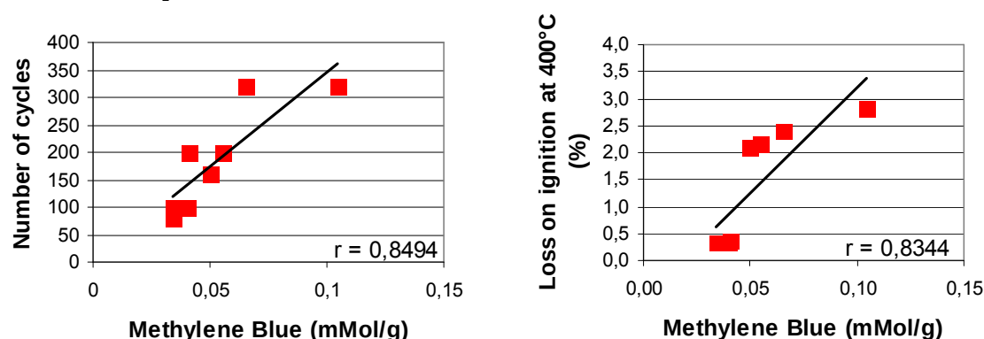
Figure 6a: Number of cycles, needed to compact the asphalt concrete specimens, as a function of methylene blue value.
